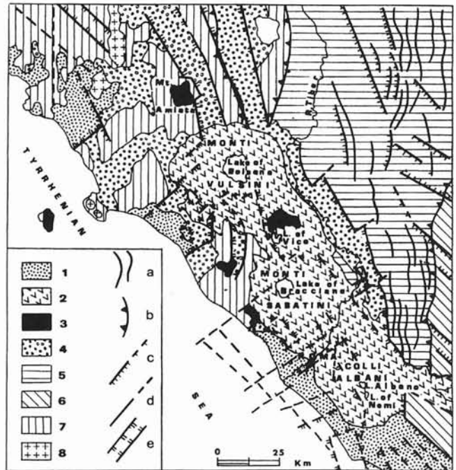
FIG. 14 - Geostructural sketch showing the tectonic arrangement in which the volcanism of Latium developed. 1) Present and recent alluvium; 2) k-alkaline volcanites; 3) plutonites and acid volcanites; 4) sands and clays neoautochthonous unit of Plio-Pleistocene; 5) Umbria-Marche sedimentary units (Trias-Upper Miocene); 6) Latium-Abruzzi carbonatic units (Trias-Upper Miocene); 7) allochthonous complexes (Sicilidi and Liguridi flysches) and Tuscan nappe; 8) Tuscan autochthonous and paraautochthonous; a) fold; b) thrust c) normal fault; d) vertical fault; e) horst-graben structure (from CAPUTO & alii, 1989).
