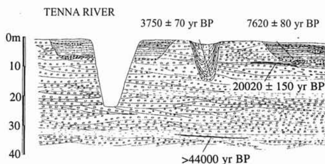
FIG. 8 - Tenna river depositional sequence (after CILLA & alii , 1996).
