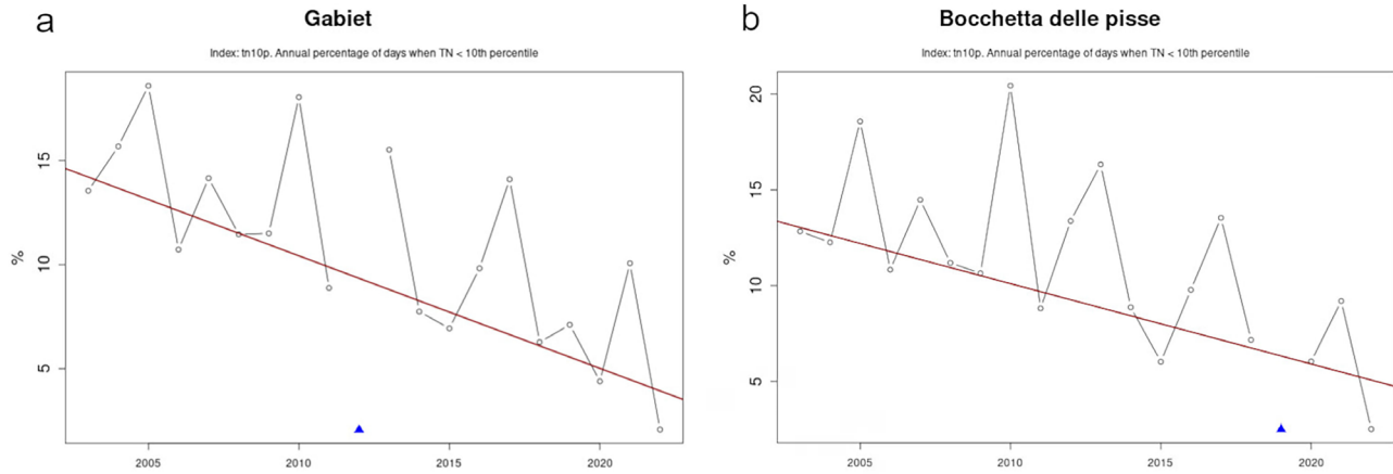
Figure 3 - Time series of the TN10p index (black line and circles) and its linear trend (red line) for the period 2003-2022. Panel a: Gabiet; Panel b: Bocchetta delle Pisse. Blue triangles symbolize missing data.
